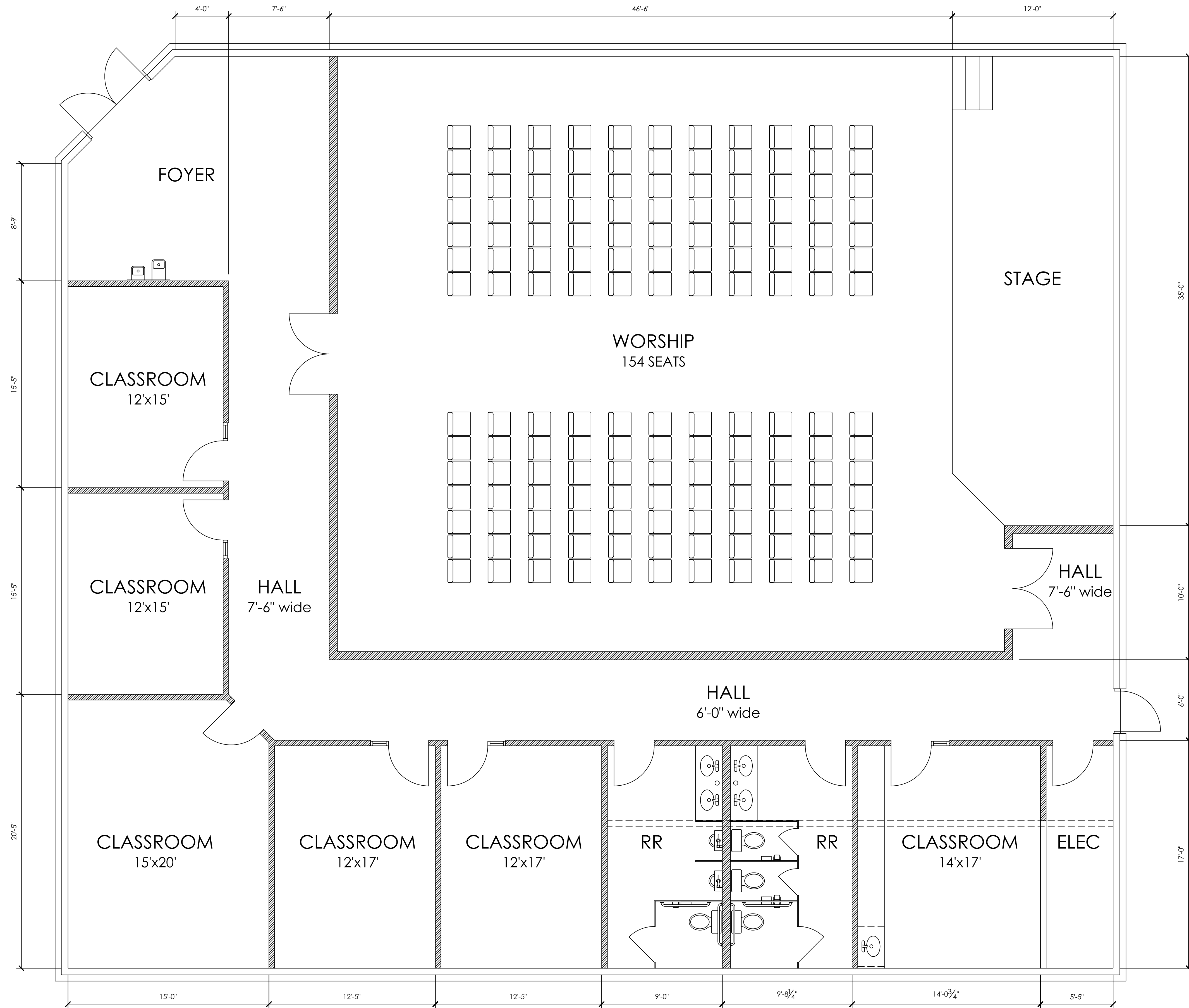
NORTH VILLAGE CHURCH FLOOR PLAN 5-5-2020
